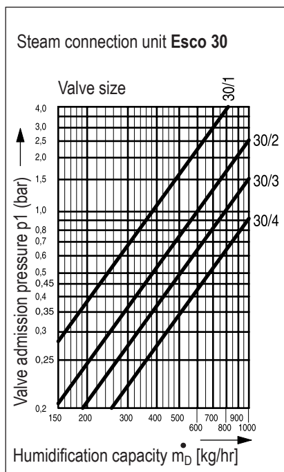
Selection diagram for dimensioning the connection unit Esco 30 with the corresponding valve size.
