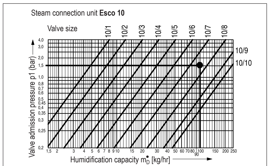
Selection diagram for dimensioning the connection unit Esco 10 with the corresponding valve size.
